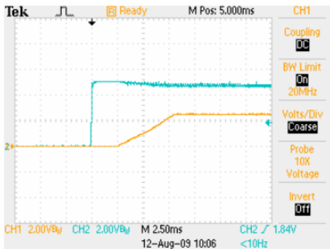
Start-up V_{IN}=5V , I_O=16A
