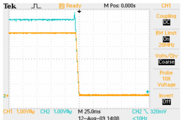
Power Down with EasyTrack™ Control V_{Track}=12V , I_O=16A Blue: EasyTrack™ Control Voltage Yellow: Output Voltage
