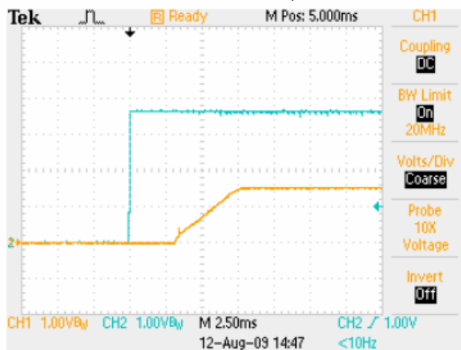
Short Circuit Protection, V_{IN}=5V
