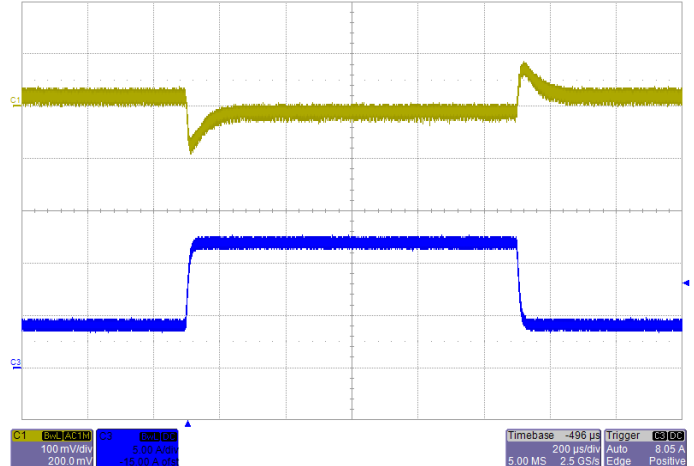
Transient Response V_{IN}=12V , Step from 4A-12A-4A, C_o=220\mu F Blue: Load Current Yellow: Output Ripple
