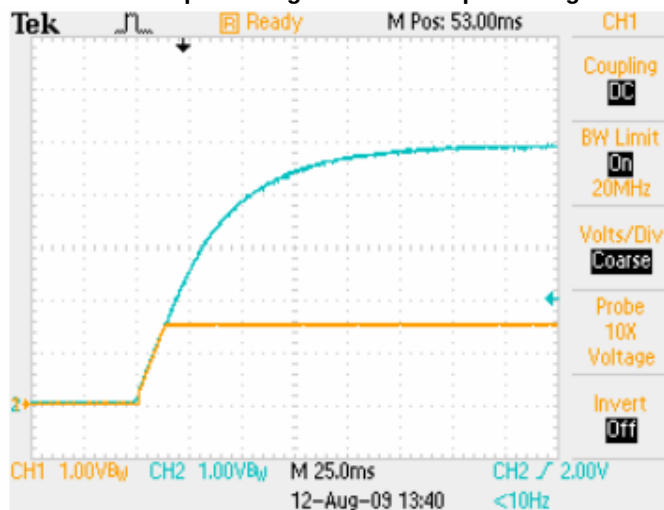
Power Up with EasyTrack™ Control V_{Track}=5.0V , I_O=16A Blue: EasyTrack™ Control Voltage Yellow: Output Voltage
