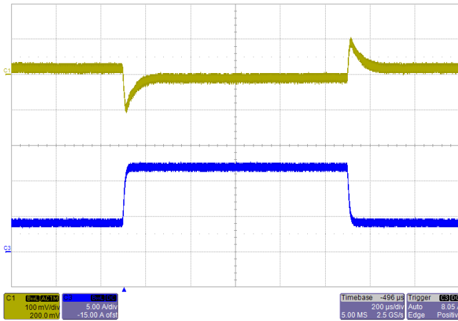
Transient Response V_{IN}=5V , Step from 4A-12A-4A, C_o=220\mu F Blue: Load Current Yellow: Output Ripple
