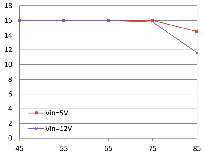
Output Current Derating (Input filter: 68 \mu F/20V TAN*5; Output filter: 226/10VCeramic*2 +220 \mu F/10V TAN*8)
