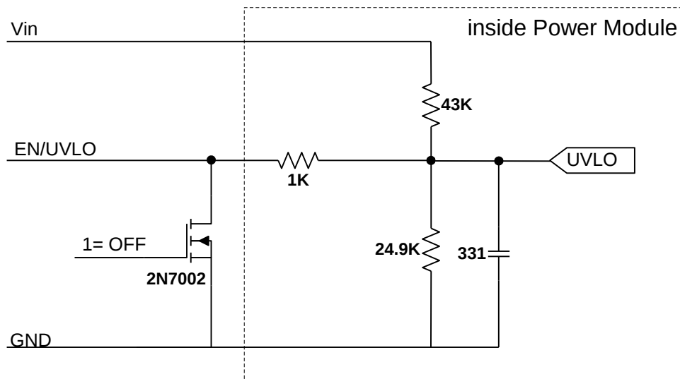
Fig5, Output ON/OFF Control Implementation with Open Drain transistor
