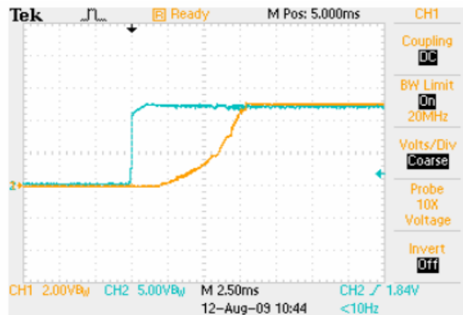
Start-up V_{IN}=12V , I_O=16A Yellow: Output Voltage Blue: Input Voltage
