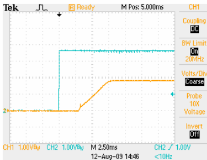
Power Up with ON/OFF Control, V_{IN}=5V
