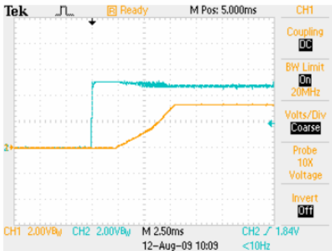
Start-up V_{IN}=5V , I_O=16A Yellow: Output Voltage Blue: Input Voltage
