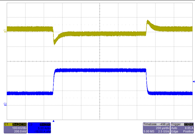
Transient Response V_{IN}=12V , Step from 4A-12A-4A, C_o=220\mu F
