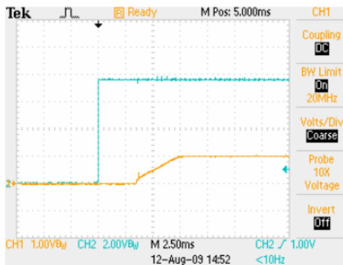
Power Up with ON/OFF Control, V_{IN}=11V
