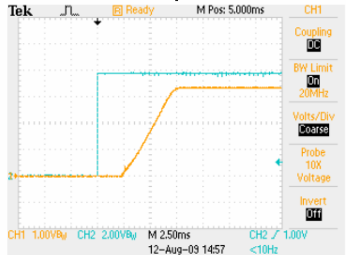
Power Up with ON/OFF Control, V_{IN}=12V
