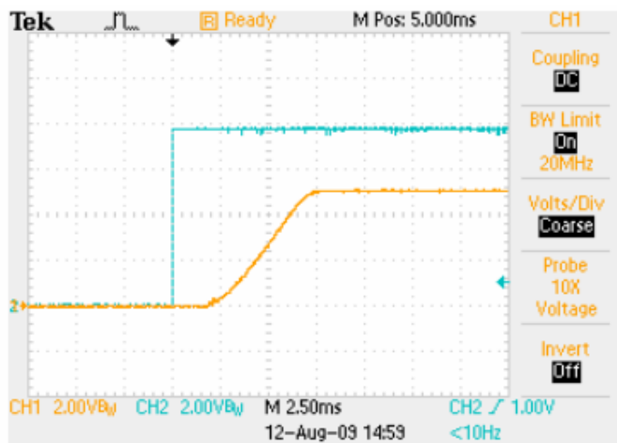
Power Up with ON/OFF Control, V_{IN}=12V Blue: ON/OFF Control Voltage Yellow: Output Voltage
