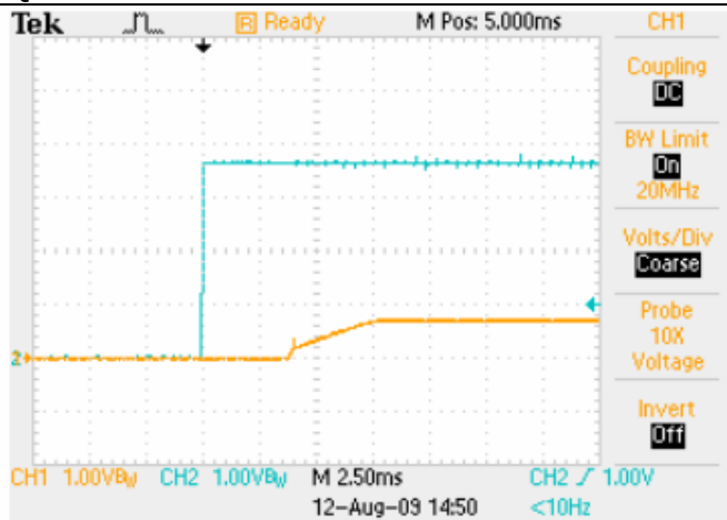
Power Up with ON/OFF Control, V_{IN}=5V Blue: ON/OFF Control Voltage Yellow: Output Voltage
