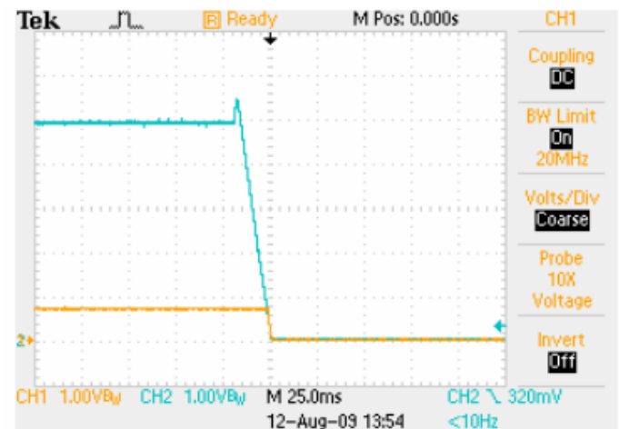
Power Down with EasyTrack™ Control V_{Track}=5V , I_O=16A Blue: EasyTrack™ Control Voltage Yellow: Output Voltage
