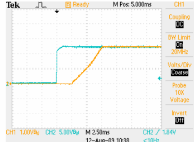
Start-up V_{IN}=12V , I_O=16A
