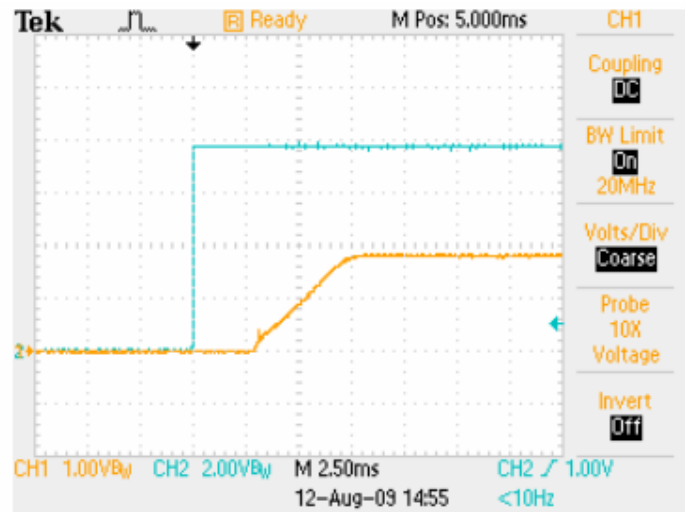
Power Up with ON/OFF Control, V_{IN}=12V
