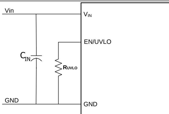
Figure 8UVLO Implementation
