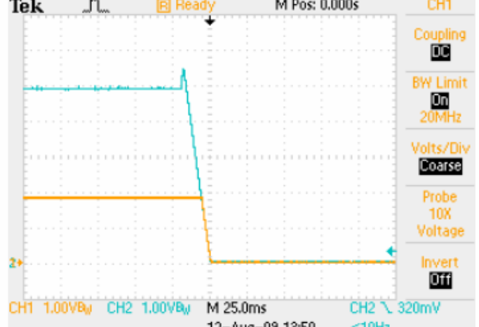
Power Down with EasyTrack™ Control V_{Track}=5V , I_O=16A Blue: EasyTrack™ Control Voltage Yellow: Output Voltage
