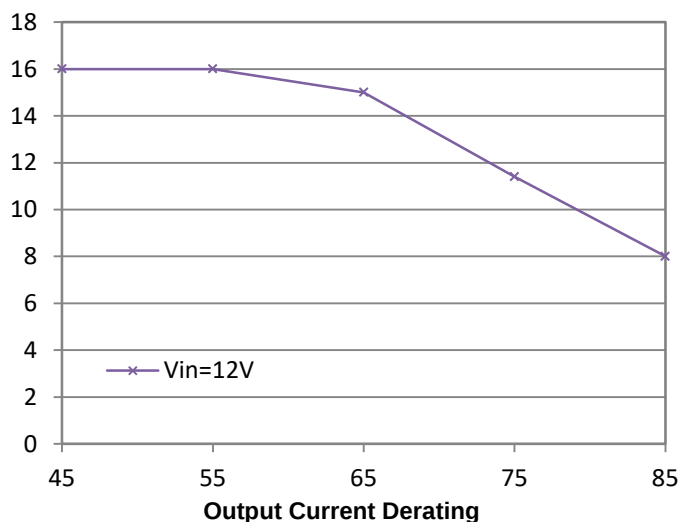
Output Current Derating (Input filter: 68 \mu F/20V TAN*5; Output filter: 226/10VCeramic*2 +220 \mu F/10V TAN*8)
