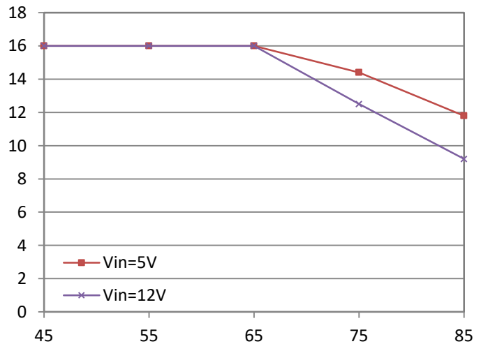
Output Current Derating (Input filter: 68 \mu F/20V TAN*5; Output filter: 226/10VCeramic*2 +220 \mu F/10V TAN*8)
