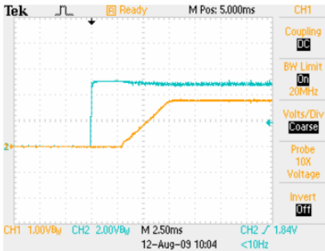
Start-up V_{IN}=5V , I_O=16A Yellow: Output Voltage Blue: Input Voltage
