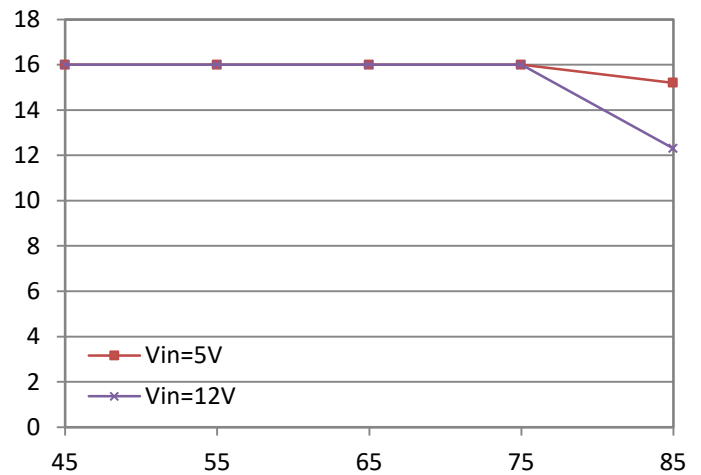
Output Current Derating (Input filter: 68 \mu F/20V TAN*5; Output filter: 226/10VCeramic*2 +220 \mu F/10V TAN*8)
