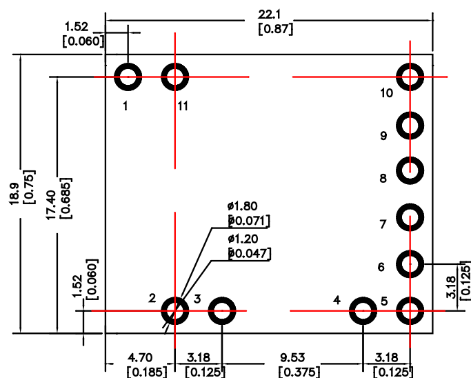
Component-side footprint
