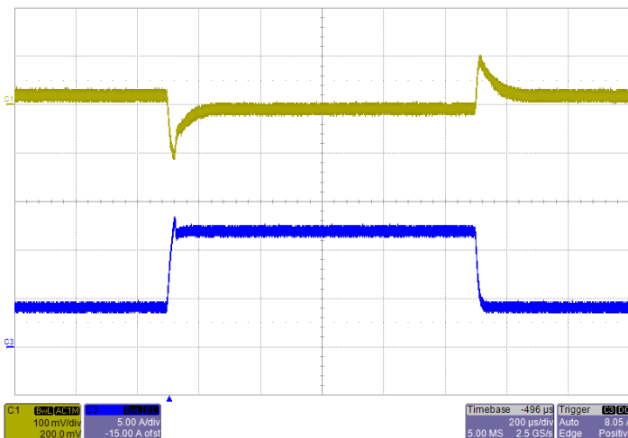
Transient Response V_{IN}=5V , Step from 4A~12A~4A, C_o=220\mu F
