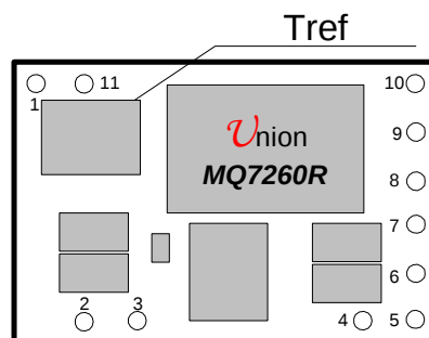
Fig 6, Temperature Reference Point
