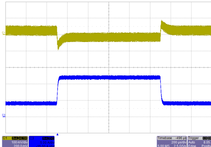
Transient Response V_{IN}=12V , Step from 4A~12A~4A, C_O=2000\mu F
