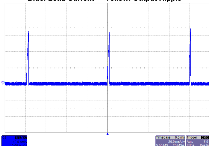
Short Circuit Protection, V_{IN}=12V
