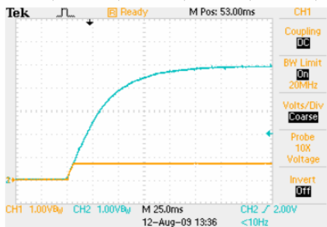
Power Up with EasyTrack™ Control V_{Track}=5.0V , I_O=16A Blue: EasyTrack™ Control Voltage Yellow: Output Voltage
