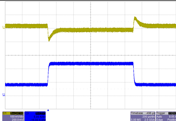
Transient Response V_{IN}=11V , Step from 4A~12A~4A, C_o=220\mu F
