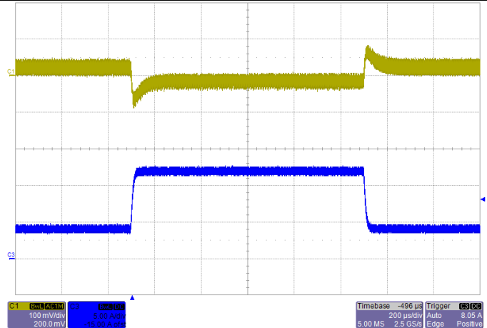
Transient Response V_{IN}=12V , Step from 4A-12A-4A, C_o=220\mu F
