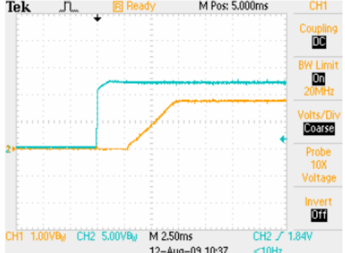
Start-up V_{IN}=12V , I_O=16A Yellow: Output Voltage Blue: Input Voltage
