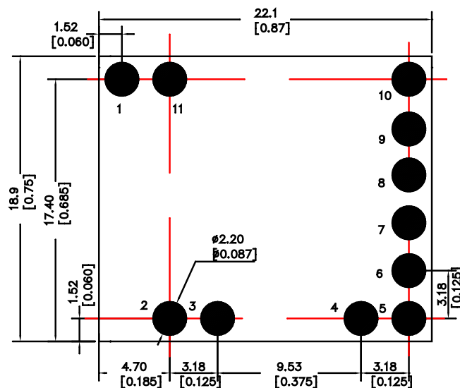
Component-side footprint
