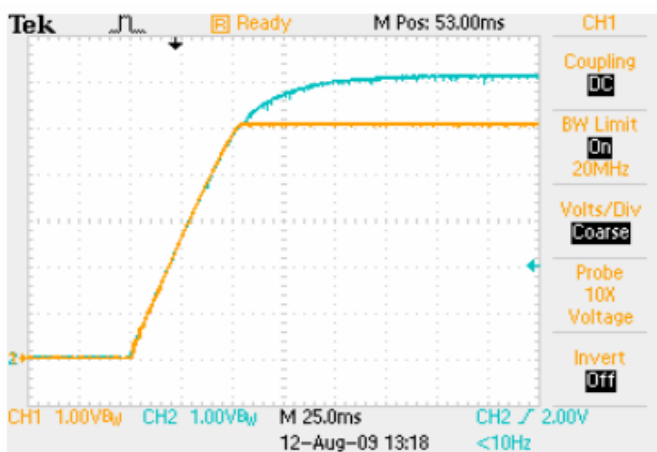
Power Up with EasyTrack™ Control V_{Track}=12V , I_O=16A Blue: EasyTrack™ Control Voltage Yellow: Output Voltage
