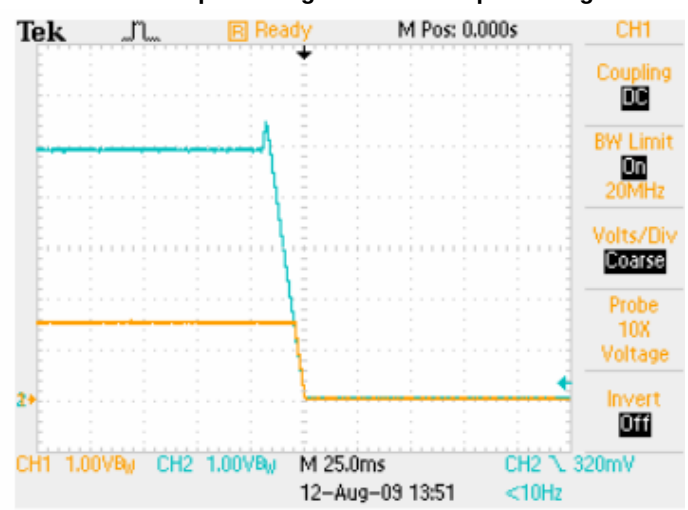
Power Down with EasyTrack™ Control V_{Track}=5V , I_O=16A Blue: EasyTrack™ Control Voltage Yellow: Output Voltage
