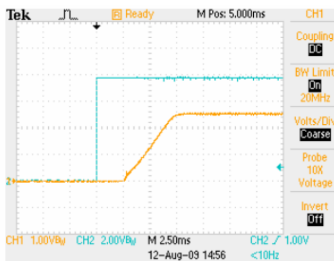
Power Up with ON/OFF Control, V_{IN}=12V
