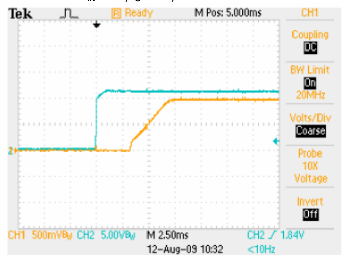
Start-up V_{IN}=11V , I_O=16A Yellow: Output Voltage Blue: Input Voltage
