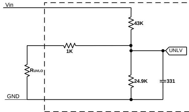
Figure 8 UVLO Implementation
