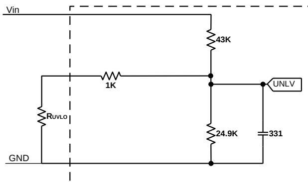
Figure 7 UVLO Implementation
