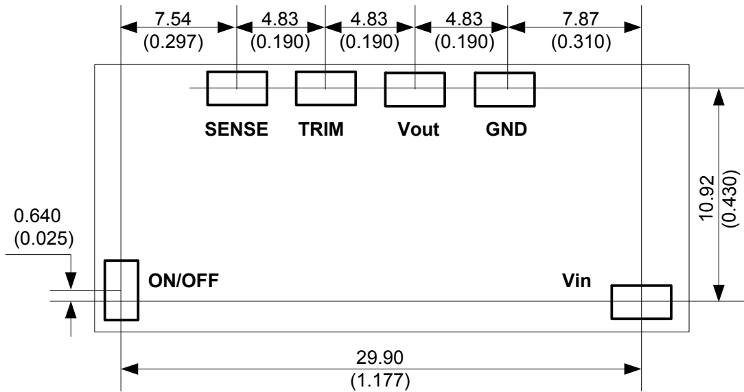
COMPONENT-SIDE FOOTPRINT
