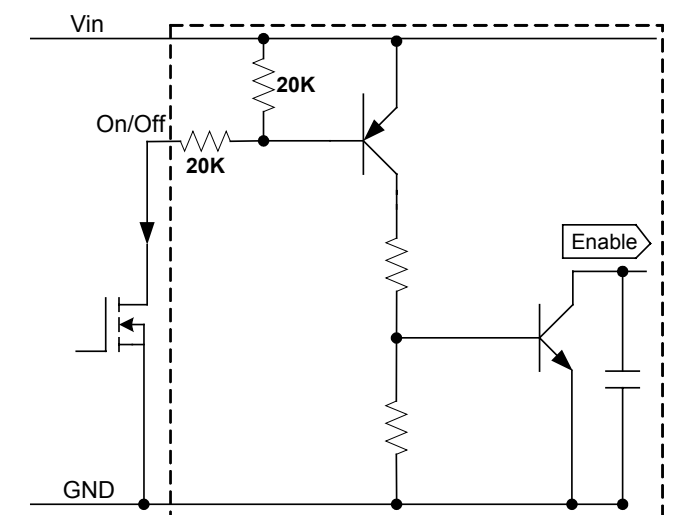
Fig1. Remote ON/OFF Implementation with pull-up pnp transistor
