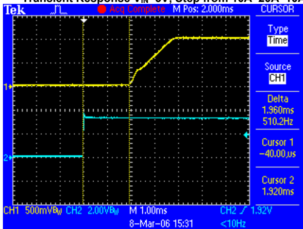
Start-up V_{IN}=3.3V , I_O=15.6A (resistive load)
