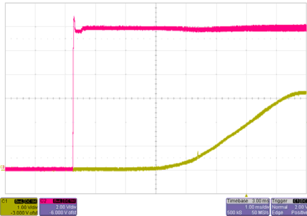
Start-up V_{IN}=12V , I_O=16A
