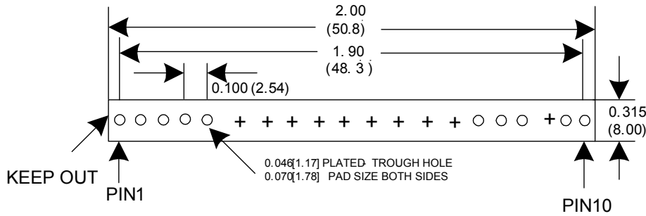
Component-side footprint
