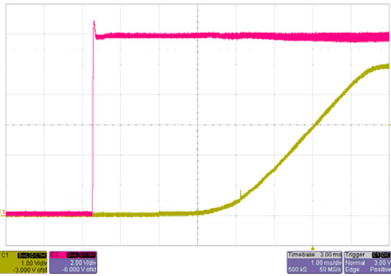
Start-up V_{IN}=12V , I_O=16A
