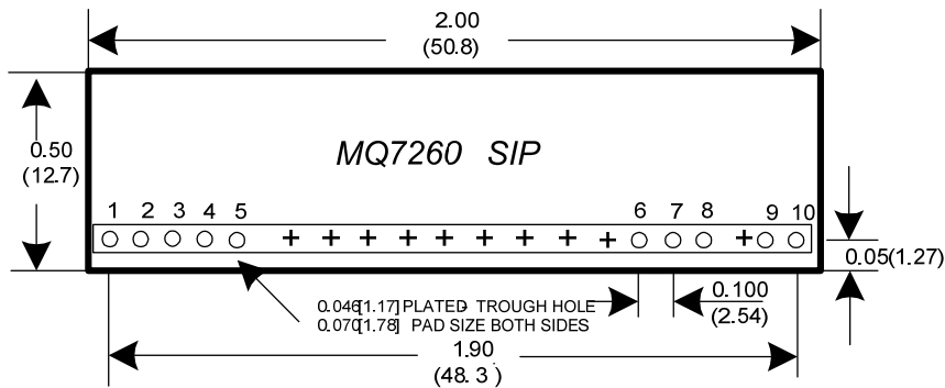
Component-side footprint
