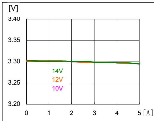
Regulation Output voltage vs. Load Current
