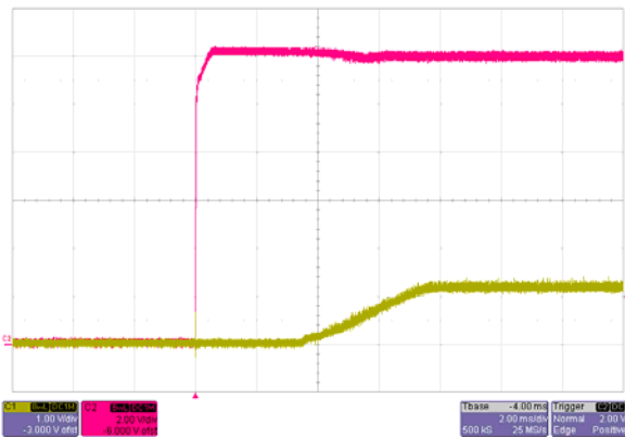
Start-up V_{IN}=12V , I_O=6A
