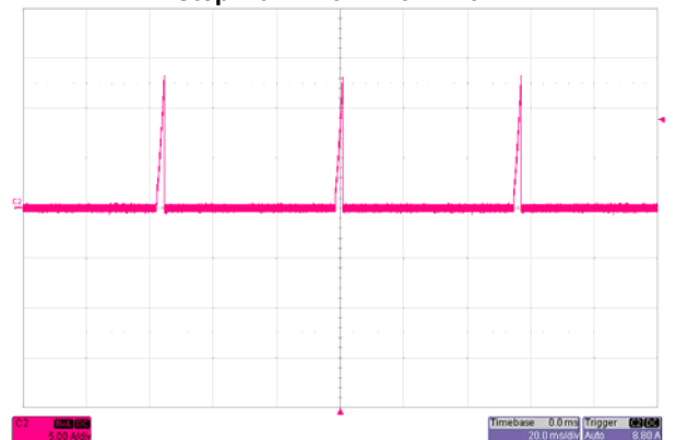
Short-Circuit Output V_{IN}=12V
