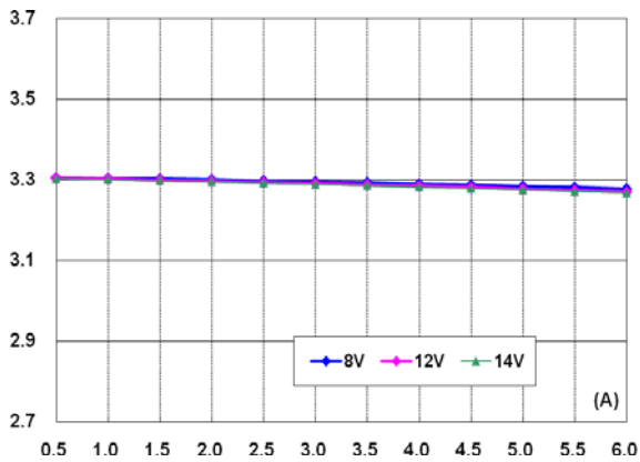
Regulation Output voltage vs. Load Current
