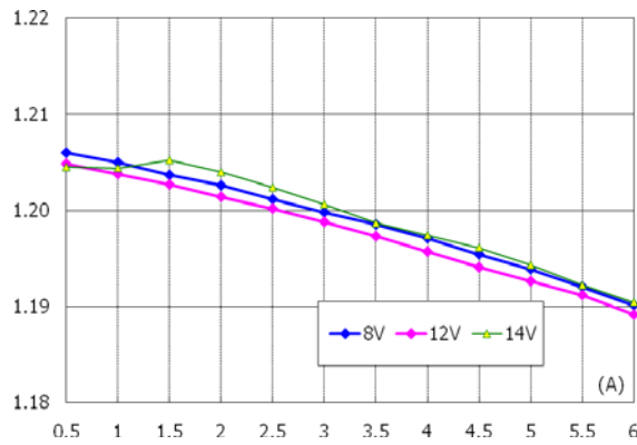
Regulation Output voltage vs. Load Current
