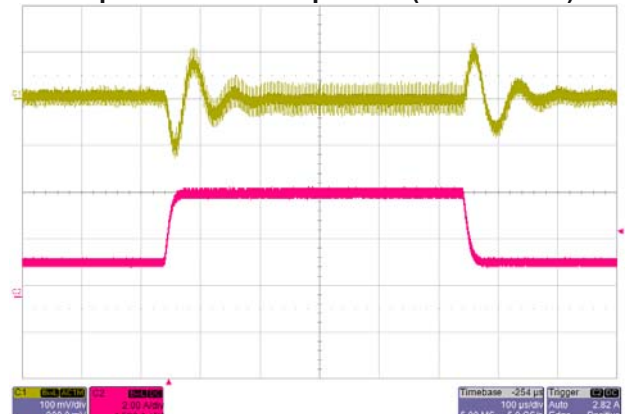
Transient Response V_{IN}=12V , Step from 1.5A~4.5A~1.5A
