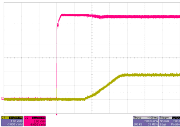
Start-up V_{IN}=12V , I_O=6A
