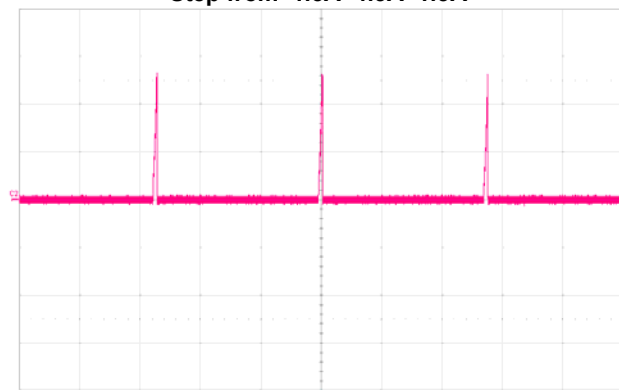
Transient Response V_{IN}=12V , Step from 1.5A~4.5A~1.5A
