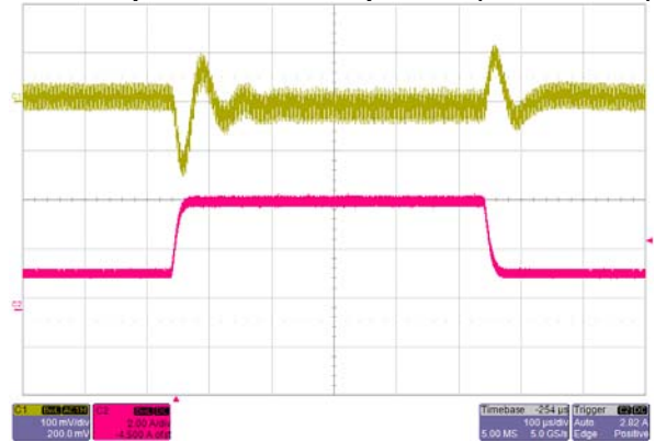
Transient Response V_{IN}=12V , Step from 1.5A~4.5A~1.5A
