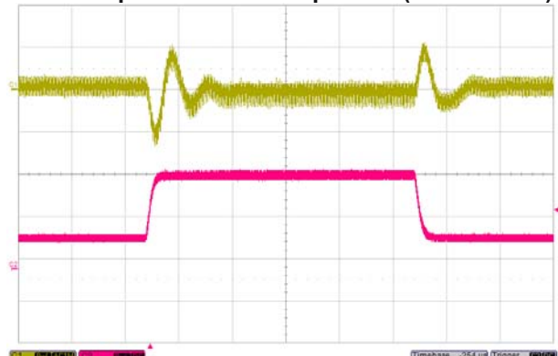
Transient Response V_{IN}=12V , Step from 1.5A~4.5A~1.5A
