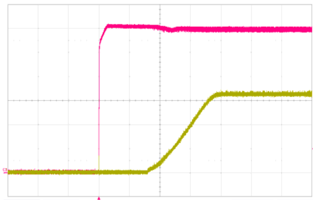
Start-up V_{IN}=12V , I_O=6A
