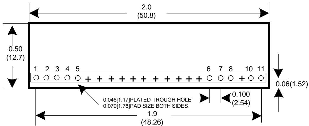
Component-side footprint
