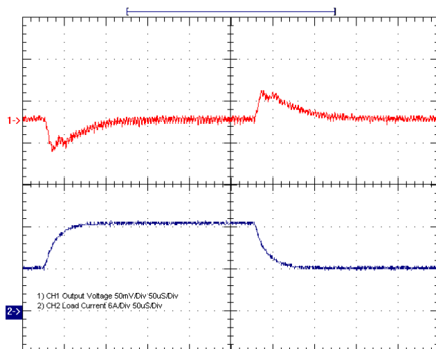
V_{IN}=3.3V, V_{OUT}=1.0V , 6A to 12A to 6A Load Step, C_{in}/C_o=0\mu F
