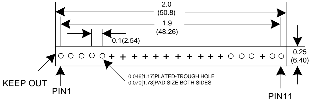
Component-side footprint
